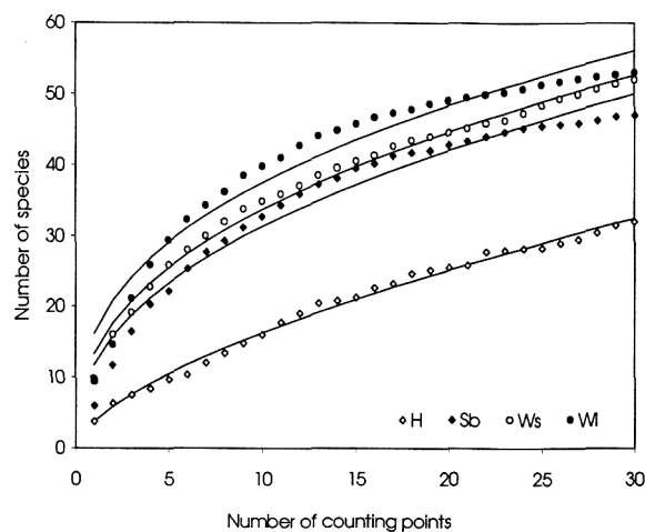
Fig. 2. Relation between the number of species and sample size in different agricultural landscapes. Dots — values observed, lines — predicted. H — homogenous farmland ( y = 3.79x^{0.63} , r^2 = 0.99 ), Sb — with shelterbelts ( y = 11.72x^{0.43} , r^2 = 0.97 ), Ws — with small woods ( y = 13.26x^{0.41} , r^2 = 0.99 ), WI — with large woods ( y = 16.13x^{0.37} , r^2 = 0.95 ).
