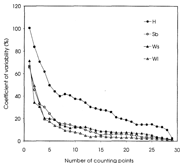
Fig. 3. Relation between coefficient of variability of species numbers and sample size in different agricultural landscapes. H — homogenous farmland, Sb — with shelterbelts, Ws — with small woods, WI — with large woods.
